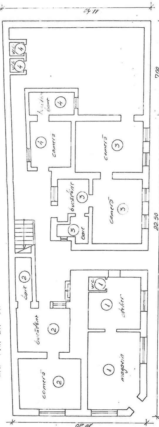
PLAN PARTER sc. 1:100
